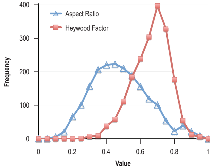
Figure 5. Frequency of occurrence of two shape factors for plagioclase particles in NU-LHT-2M. The distributions for all minerals combined is almost visually identical with the distributions shown here.
